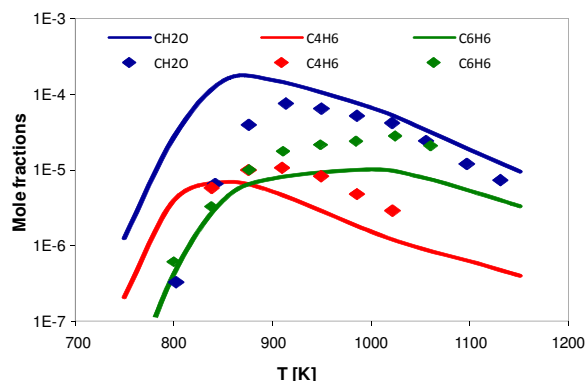
Figure 7: Experimental and calculated species profiles in a JSR (10MPa, \tau=0.5\text{s} )
