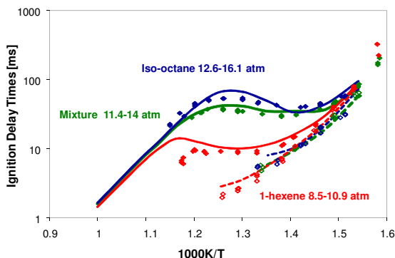
Figure 4: Ignition delay times (solid) and cool flames (dotted) of the 1-hexene/iso-octane mixture and its pure components
